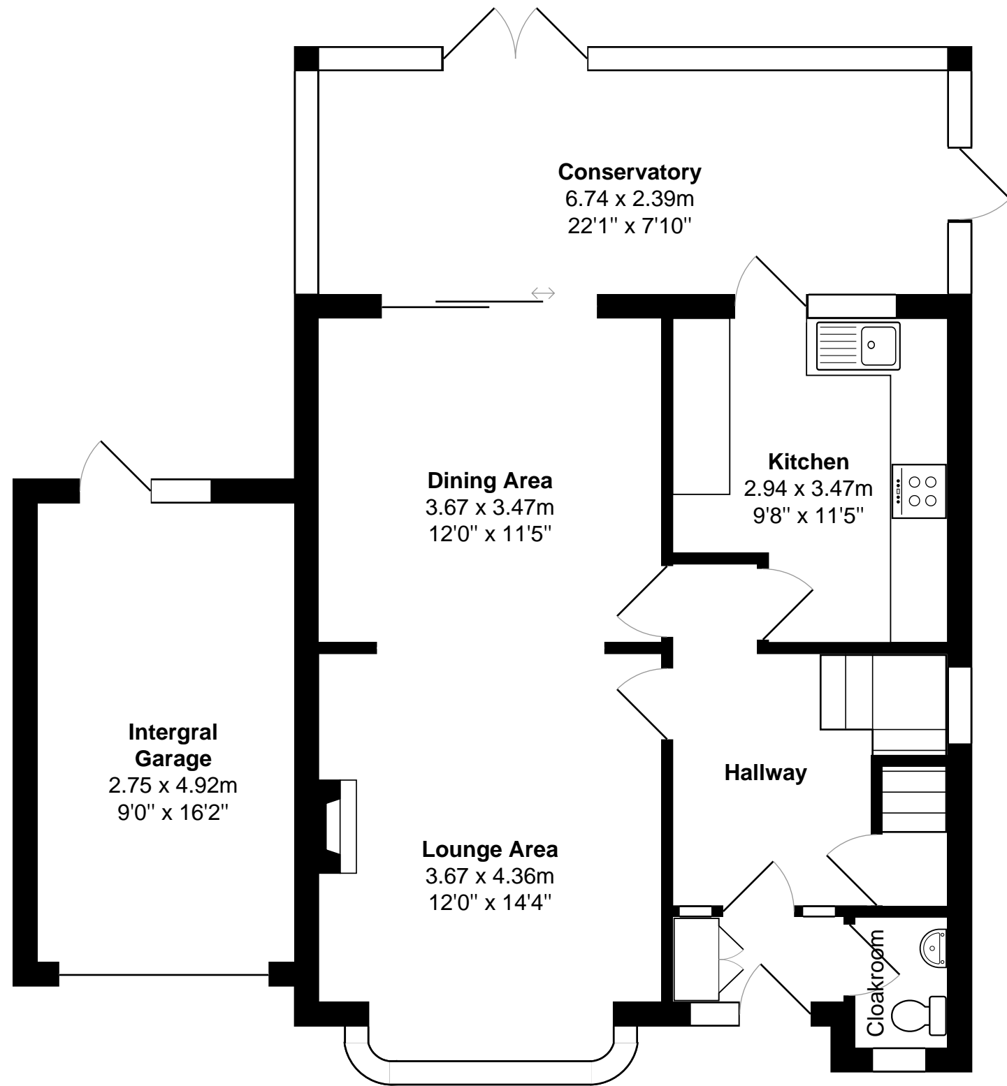
Ground Floor Area: 84.3 m 2 ... 907 ft 2
